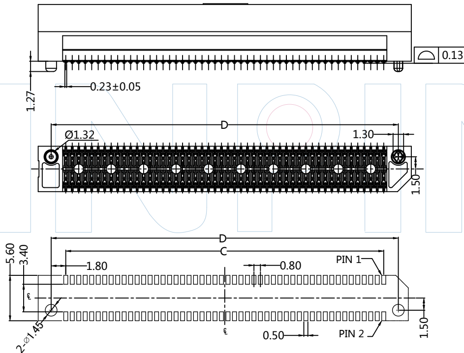
Recommended PC Board Pattern ( TOP VIEW )
